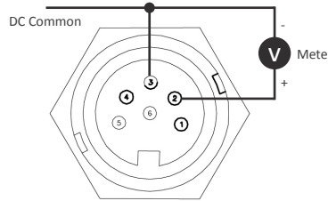
Analog Monitor-Voltage
